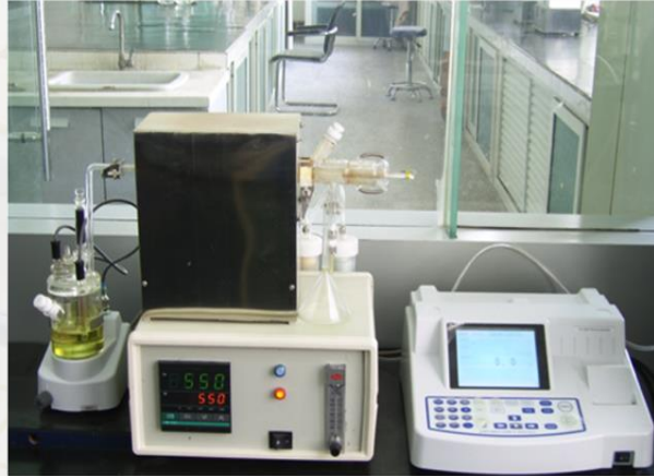
Surface area and porosity tester - Carl Fischer moisture detector BET gas adsorption tester
